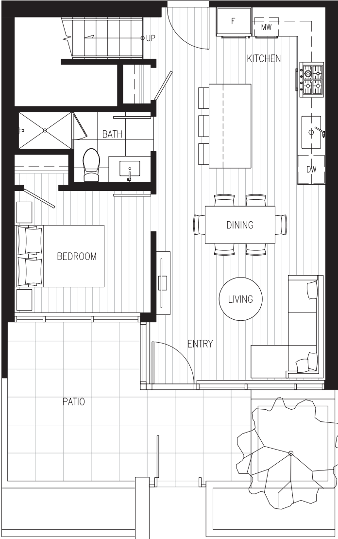
LOWER LEVEL
